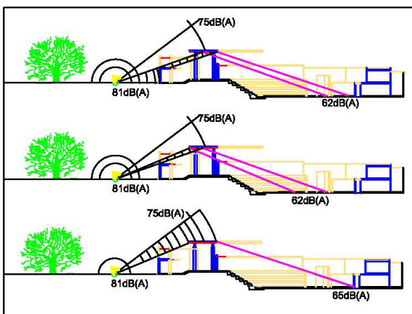
Fig.4 Section of the acoustic model. The non-efficacy of the barriers to the heavy traffic from the neighbouring street
